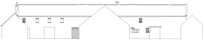
SECTION EE
